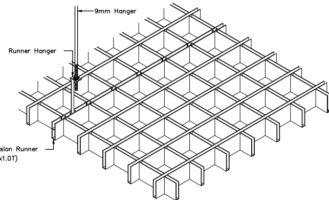
3 OPEN CELL CEILING PERSPECTIVE
