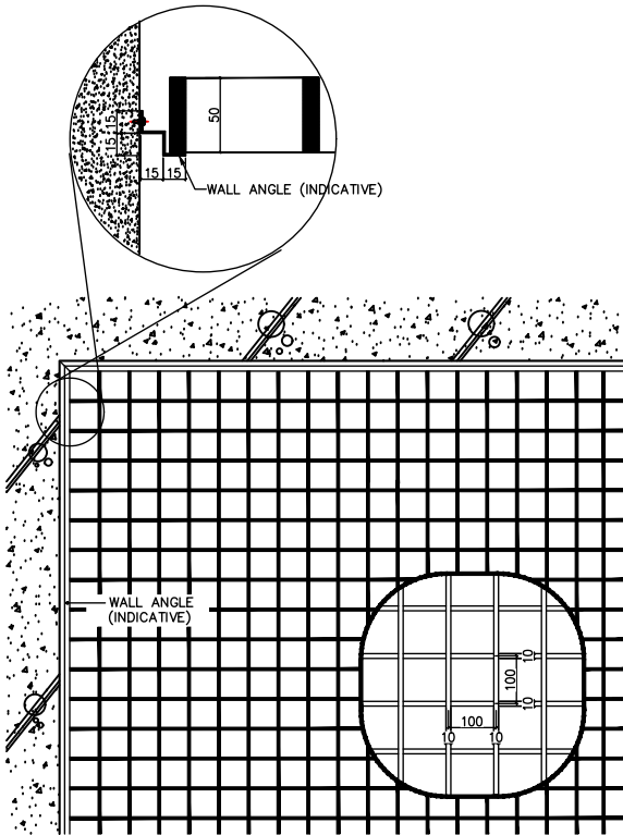
1 OPEN CELL CEILING PLAN (100X100)
