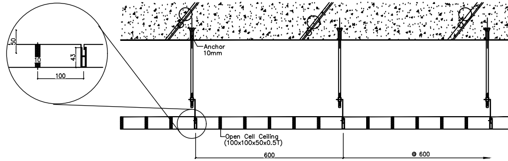
2 OPEN CELL CEILING SECTION
